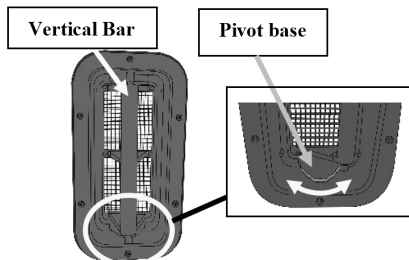
Vent port closed (Interior)
