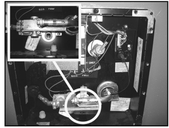
Water heater drain plug
